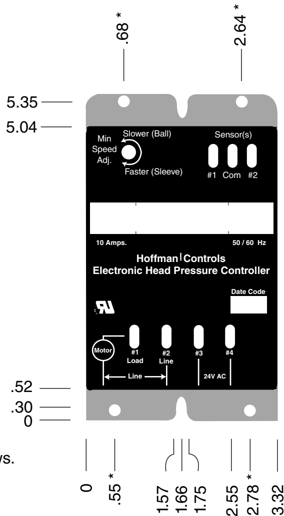
816-10D Series Control Dimensions
