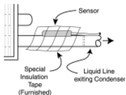
Figure 1 - Sensor Installation
